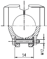
Flag Type 6300A Mat. Brass
