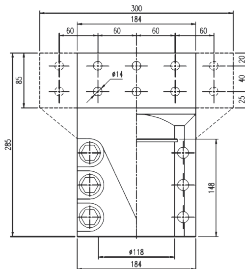
Flag Type 12500A Mat.Alu Bronze
