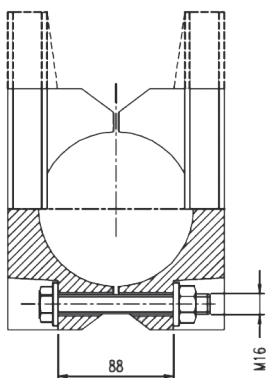
Flag Type 12500A Mat.Alu Bronze
